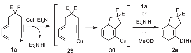
Scheme 4. Deuteration experiment which indicates that a vinylcopper intermediate may react with different proton sources to close the catalytic cycle; 90 % ([D]- 2a /H- 2a ca. 4:1).
