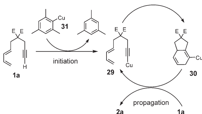
Scheme 5. Proposed catalytic cycle upon the use of mesitylcopper ( 31 ).
