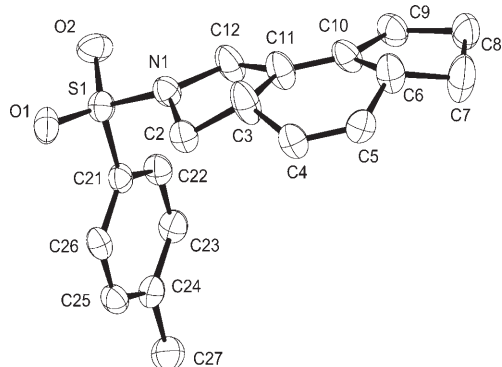
Figure 1. One of the two independent molecules of 35 in the solid state. Anisotropic displacement parameters are drawn at the 50% probability level.
