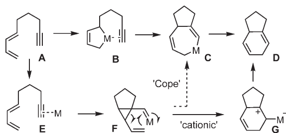
Scheme 1. Different scenarios for metal-catalyzed Diels–Alder reactions of dienynes. Top: conventional pathway based on oxidative cyclization; bottom: novel electrophilic activation manifold.
