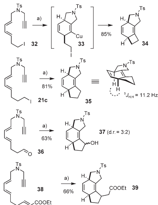
Scheme 6. Copper-mediated Diels–Alder/alkylation cascade; a) mesitylcopper ( 31 , 1 equiv), THF, -78^{\circ}\text{C} \rightarrow \text{RT} .
