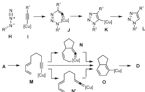
Scheme 3. Tentative mechanism of copper-catalyzed azide cycloadditions [10] and the envisaged Diels–Alder manifold involving analogous copper acetylide (–vinylidene) and –vinyl intermediates.
